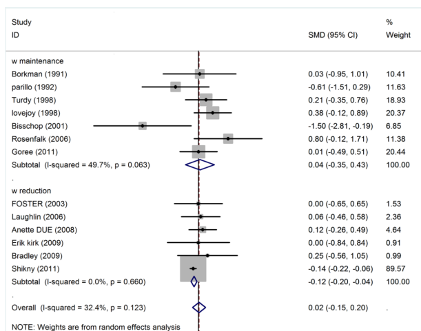
Figure 3. Forest plot showing overall effect of HFLC and LFHC diet on insulin resistance using random effects model based on weight change (with weight reduction vs weight maintenance).
