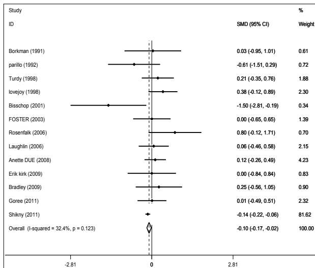
Figure 2. Forest plot showing overall effect of HFLC and LFHC diet on insulin resistance using random effects model.
